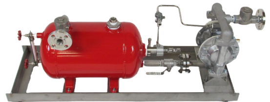
J-5000 SM-P w/1" Diaphragm Pump Skid
